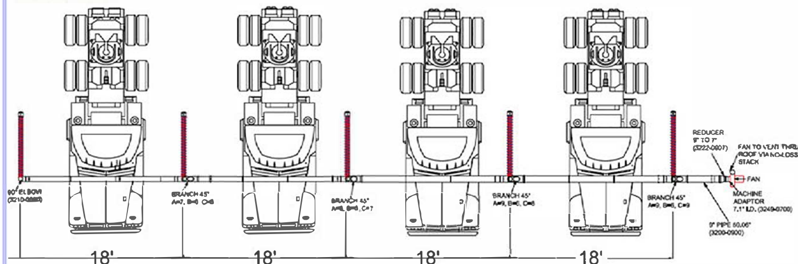
PLAN/TOP VIEW
