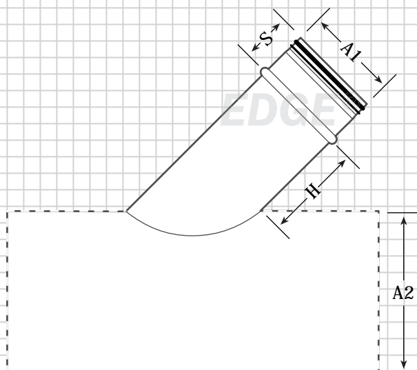
Gasket 45° Lateral (GL)
