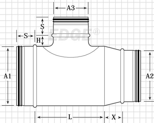
Gasket 90° Reducing Tee with Die Stamped Saddle Tap (GDSTR)
