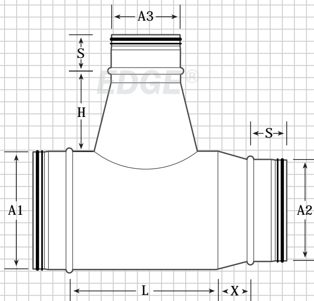
Gasket 90° Conical Reducing Tee (GCRT)
