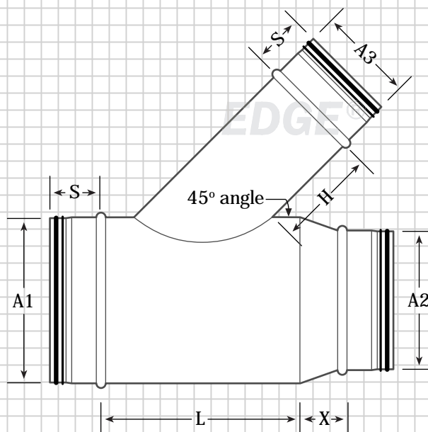
Gasket 45° Lateral Reducing Tee (GLRT)
