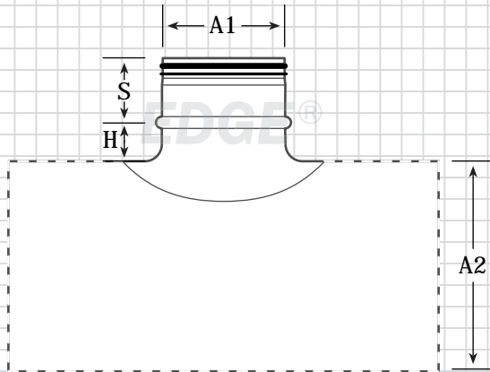
Gasket 90° Die Stamped Saddle Tap (GDST)
