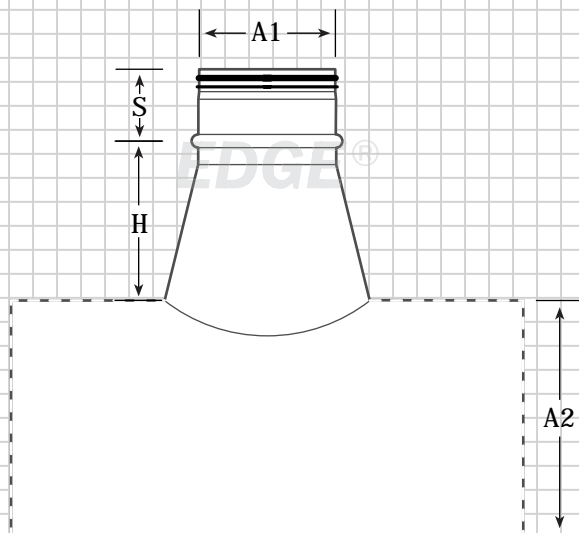
Gasket 90° Conical (GC)
