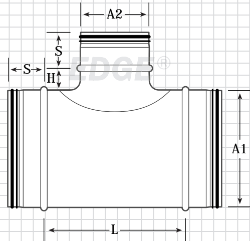
Gasket 90° Tee with Die Stamped Saddle Tap (GTDST)
