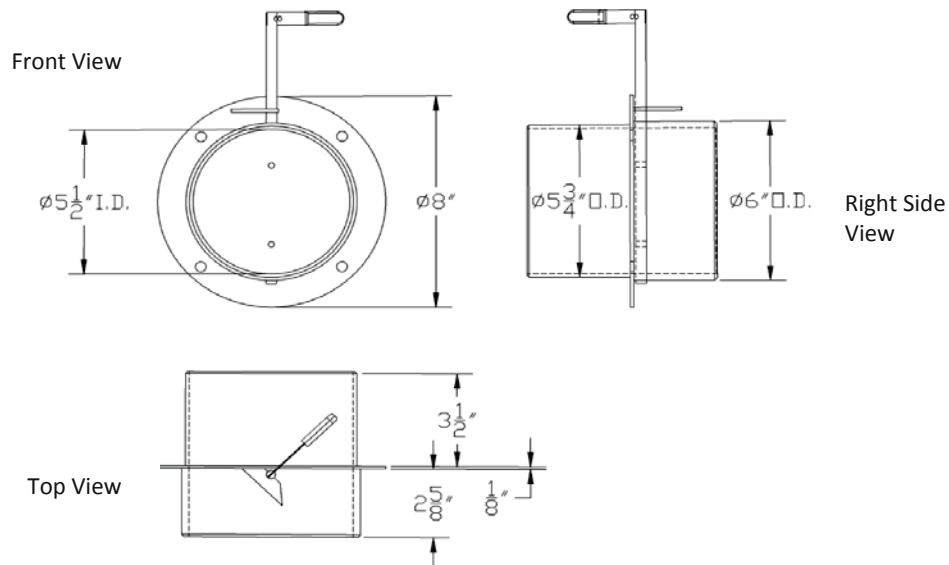
Pictured Above: The Automatic Hose Reel Mounted Damper with 6 Inch Diameter Shown Below: Orthographic Views of the Automatic Damper
